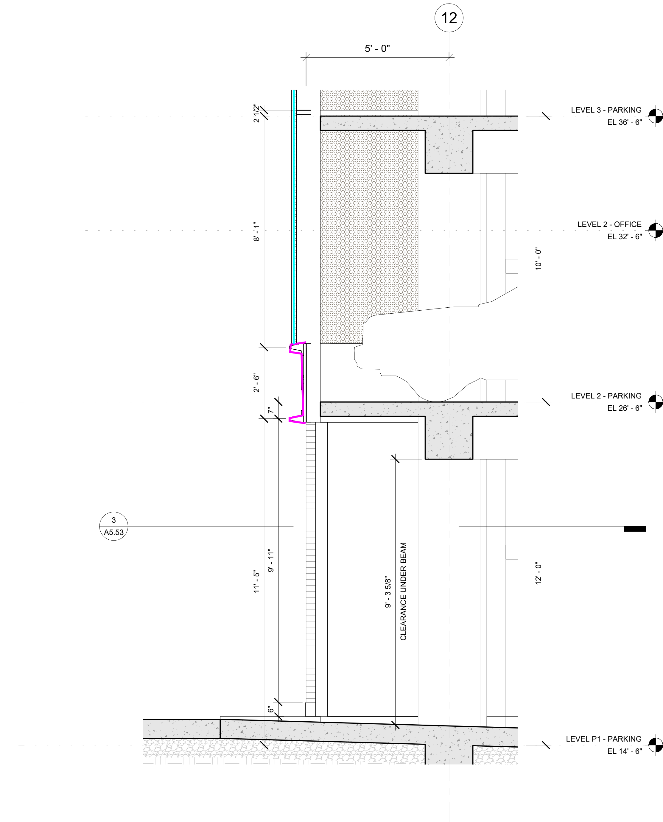
2 SECTION 1/2" = 1'-0"
